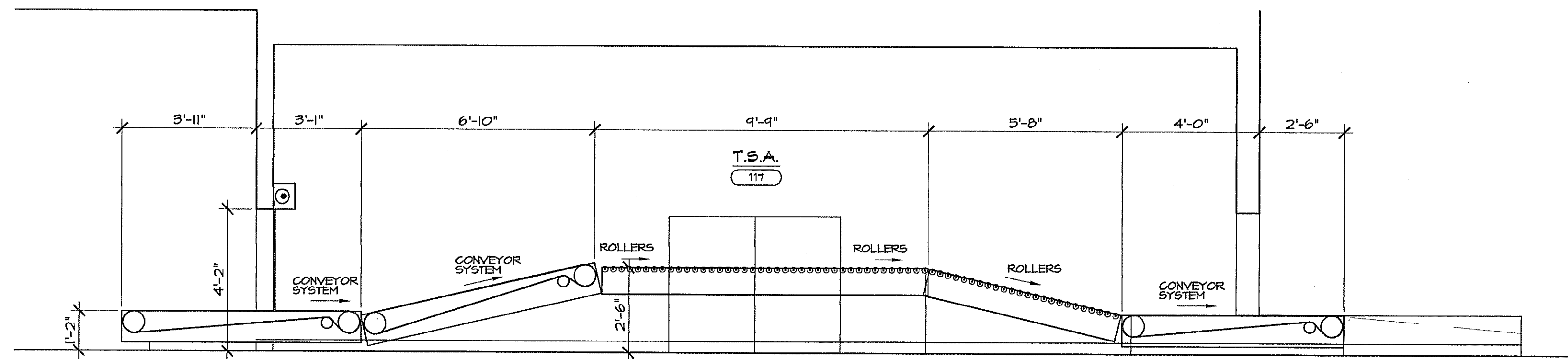
BAGGAGE CONVEYOR T.S.A. 117 SCALE: 3/8"=1'-0"
